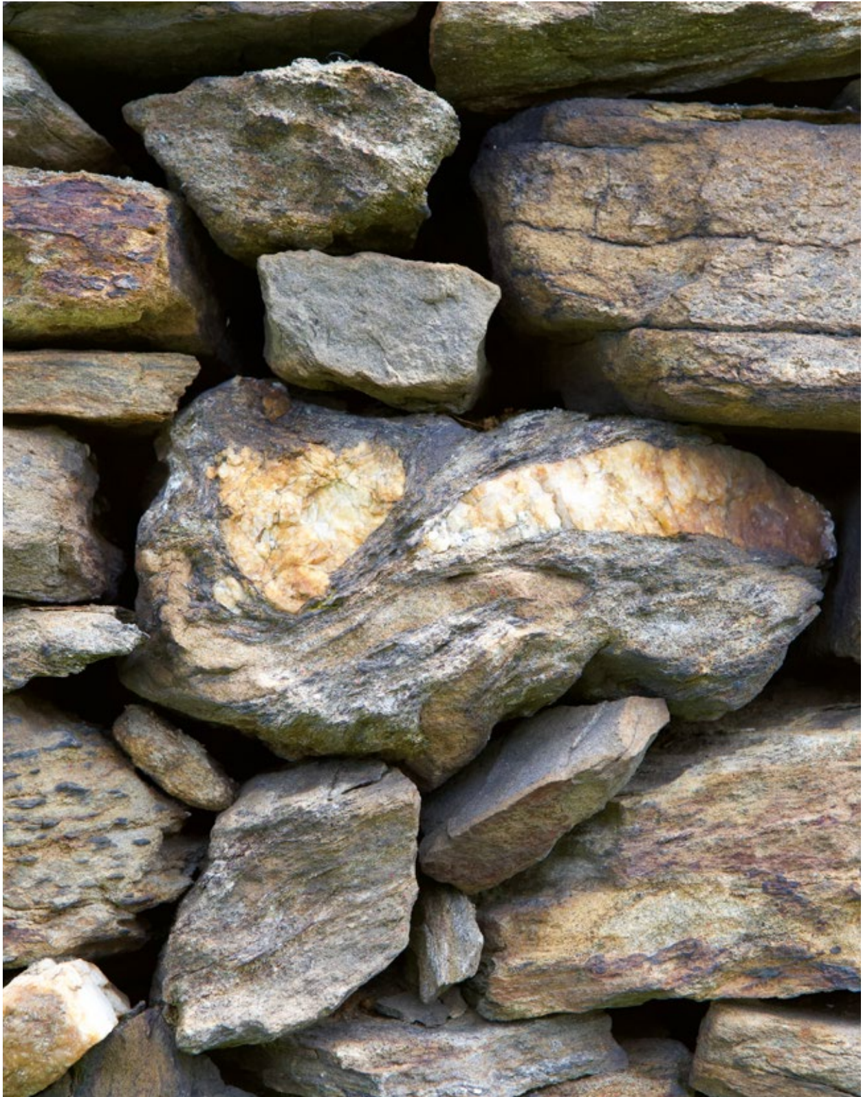
SPITZER GRABEN METAMORPHIC BEDROCK IN RIED BRANDSTATT
